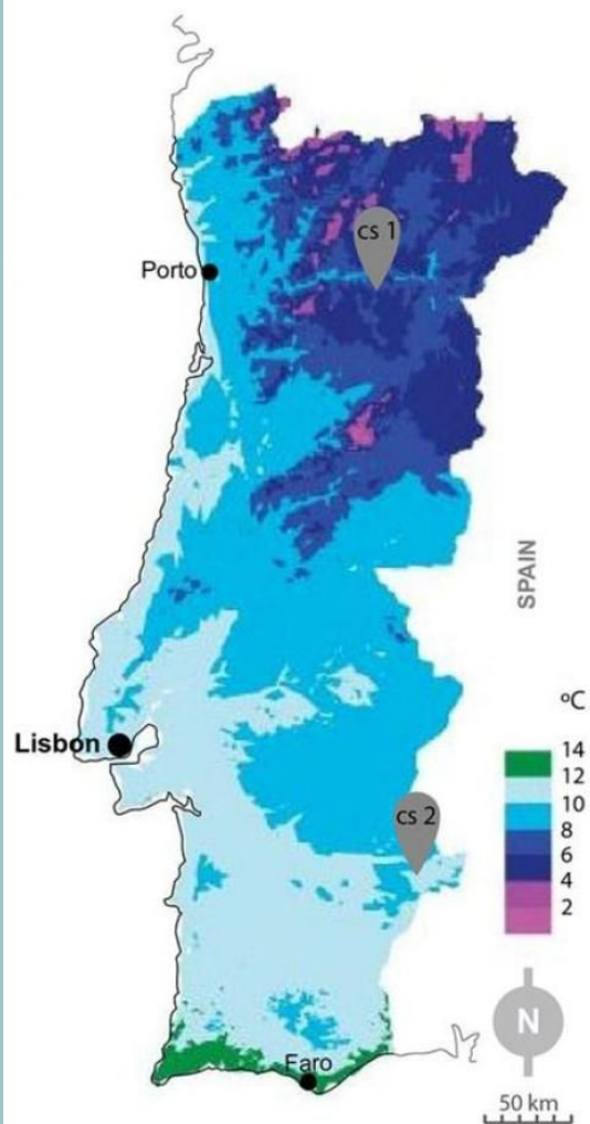
winter mean temperature
