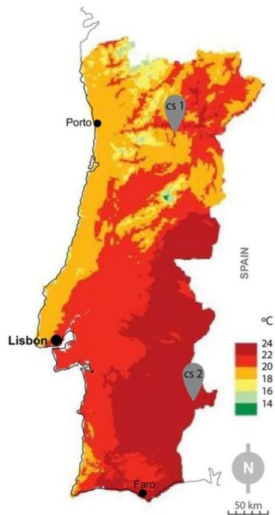
summer mean temperature
